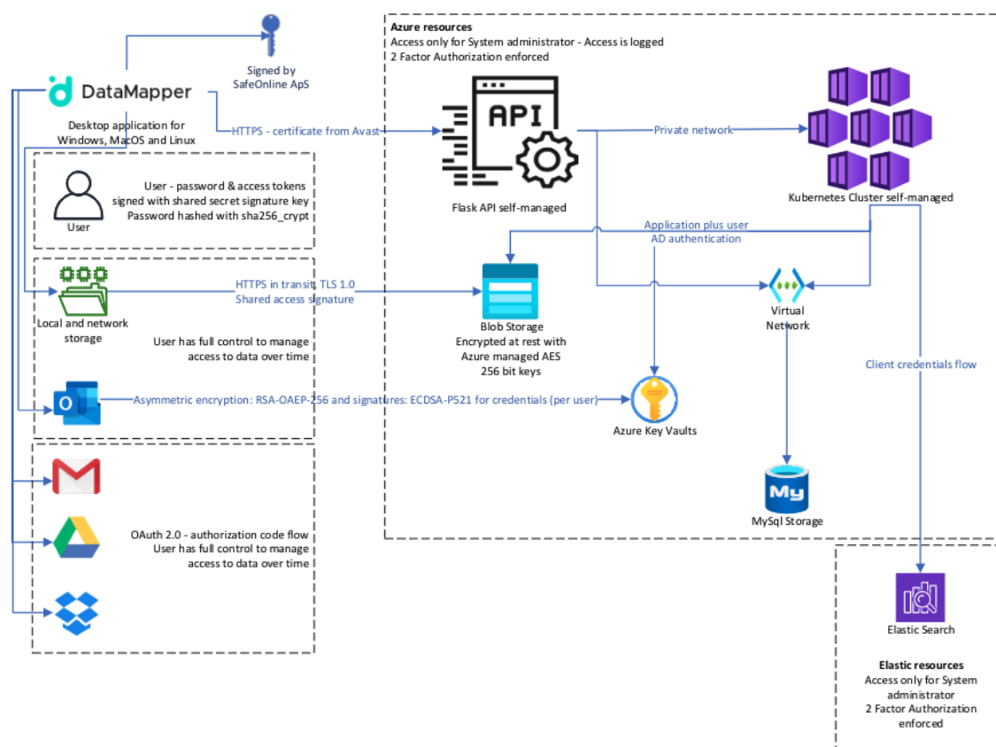
Figure 1: Connectid DataMapper, security overview
